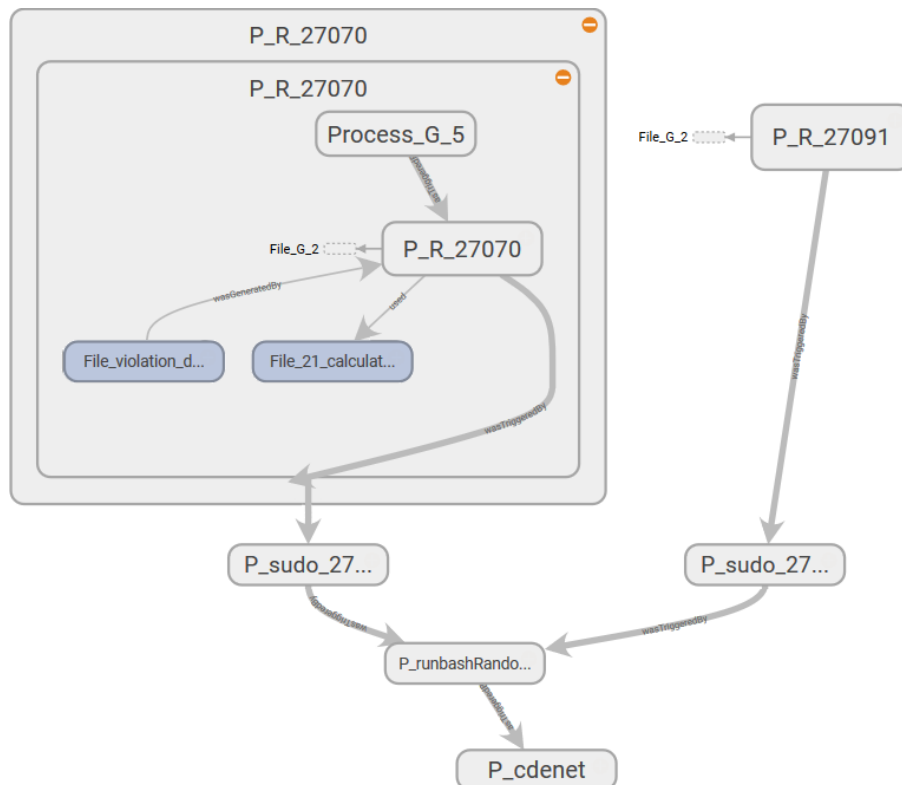
Figure 6. Expanded view of concealing node “P_R_27070” (“P_5”).
