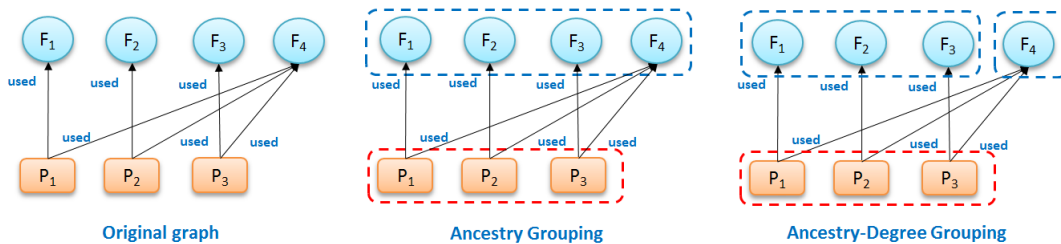
Figure 8. An example of ancestry-degree compatible grouping.
