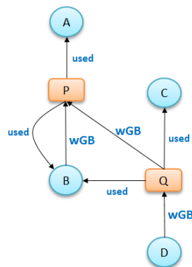
Figure 4. Provenance graph of an execution.
