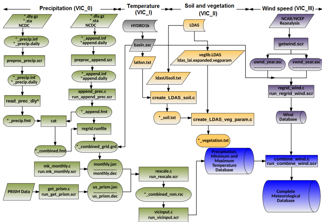
Figure 10. Conceptual view of the VIC workflow [53] ((* in this figure denotes a list of files that share the same prefix or suffix).
